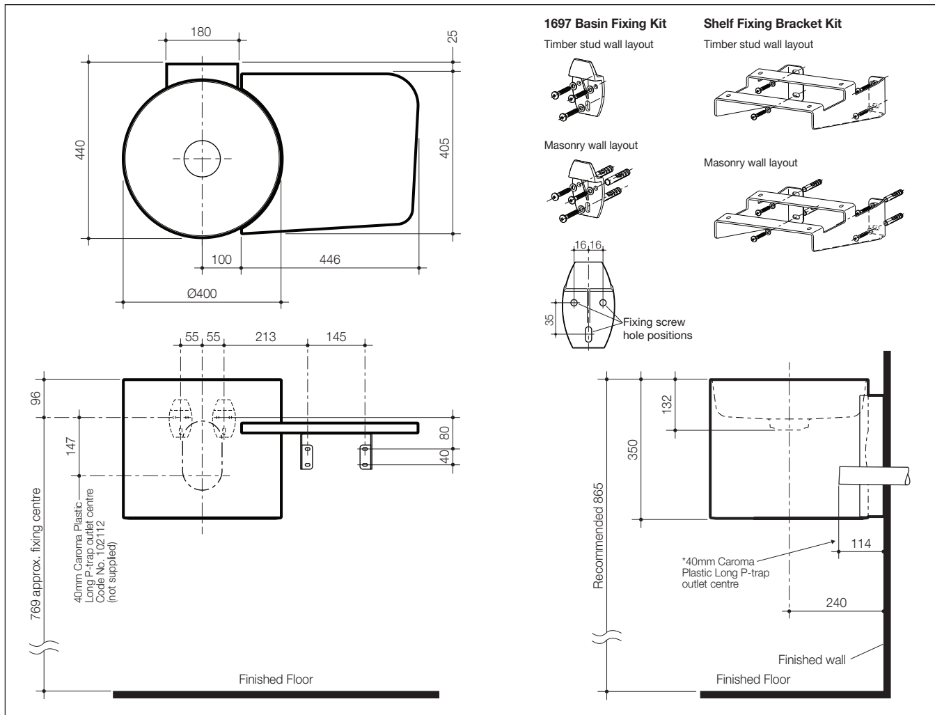
Optional right hand shelf accessory in dark wood (shelf also available in left hand)
